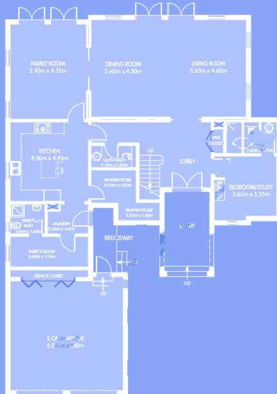
Ground Floor
