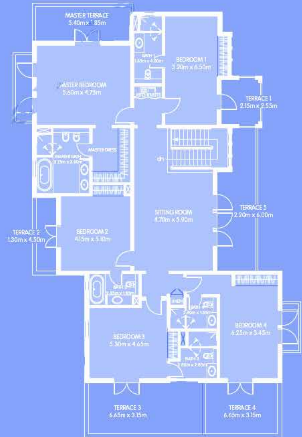
First Floor
